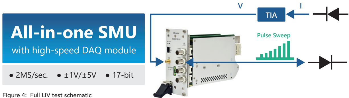
Figure 4: Full LIV test schematic
